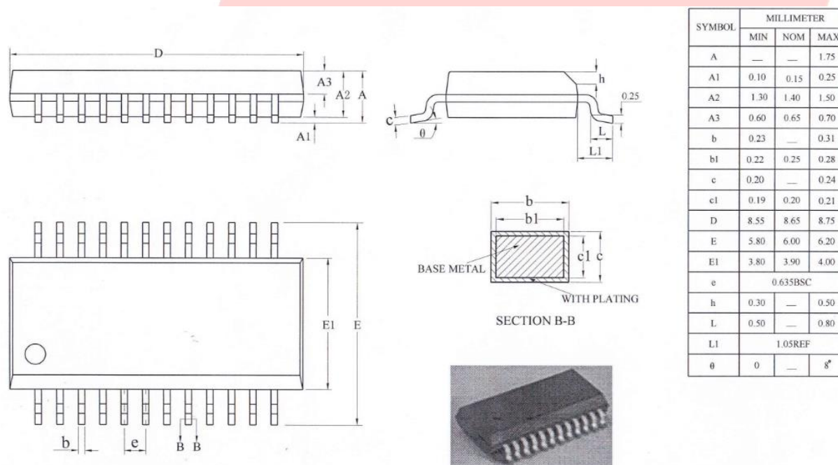
Figure 3-1. AC6925A_QSOP24 Package
